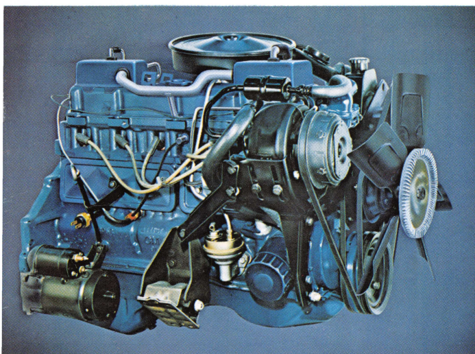
4.1 Litre (250 CID) In-Line Six gasoline engine
