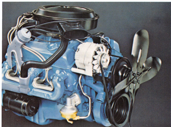
5.7 Litre (350 CID), 4-bbl., V8 gasoline engine
